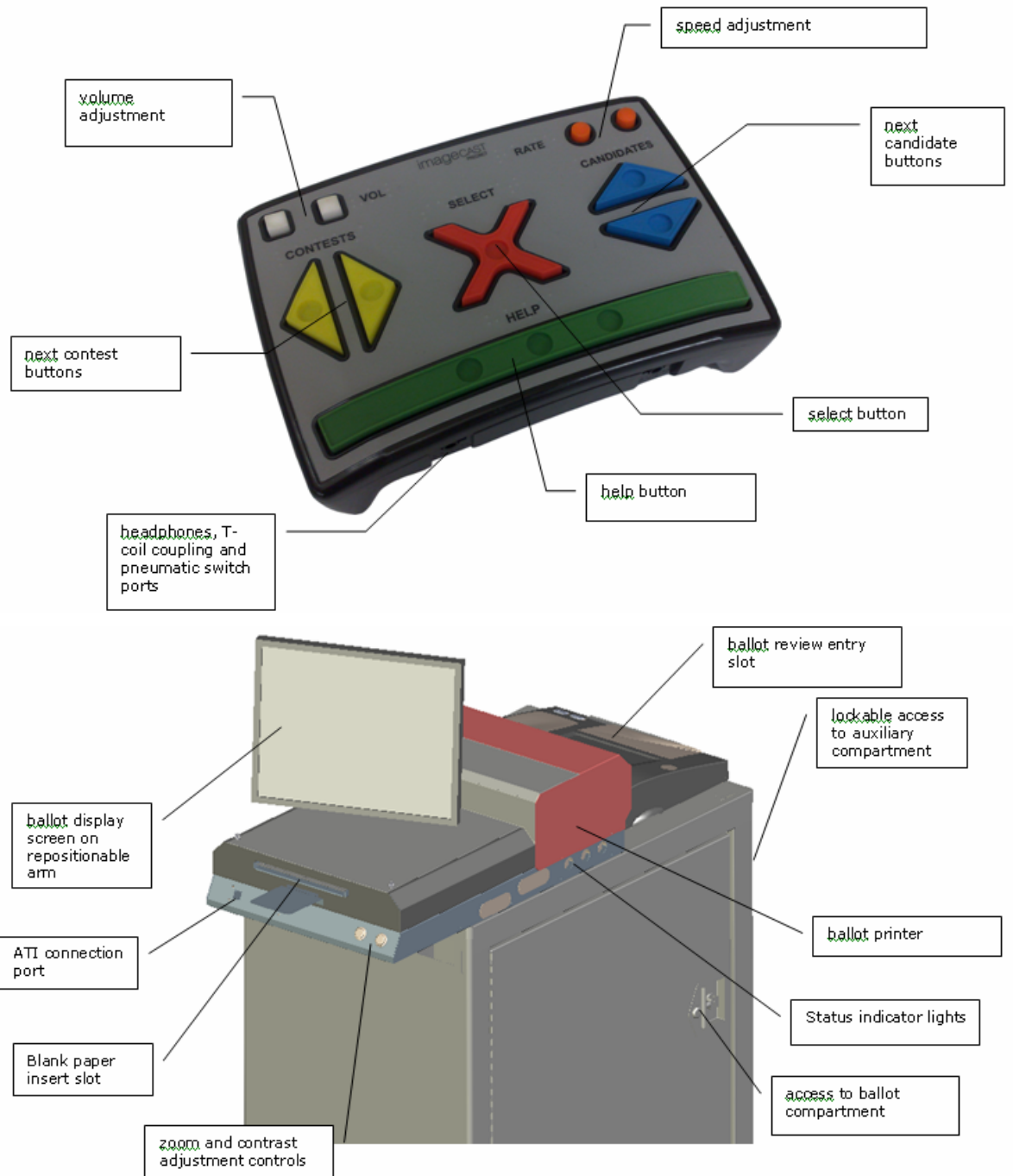
Figure 2: Audio Tactile Interface and Ballot Box
