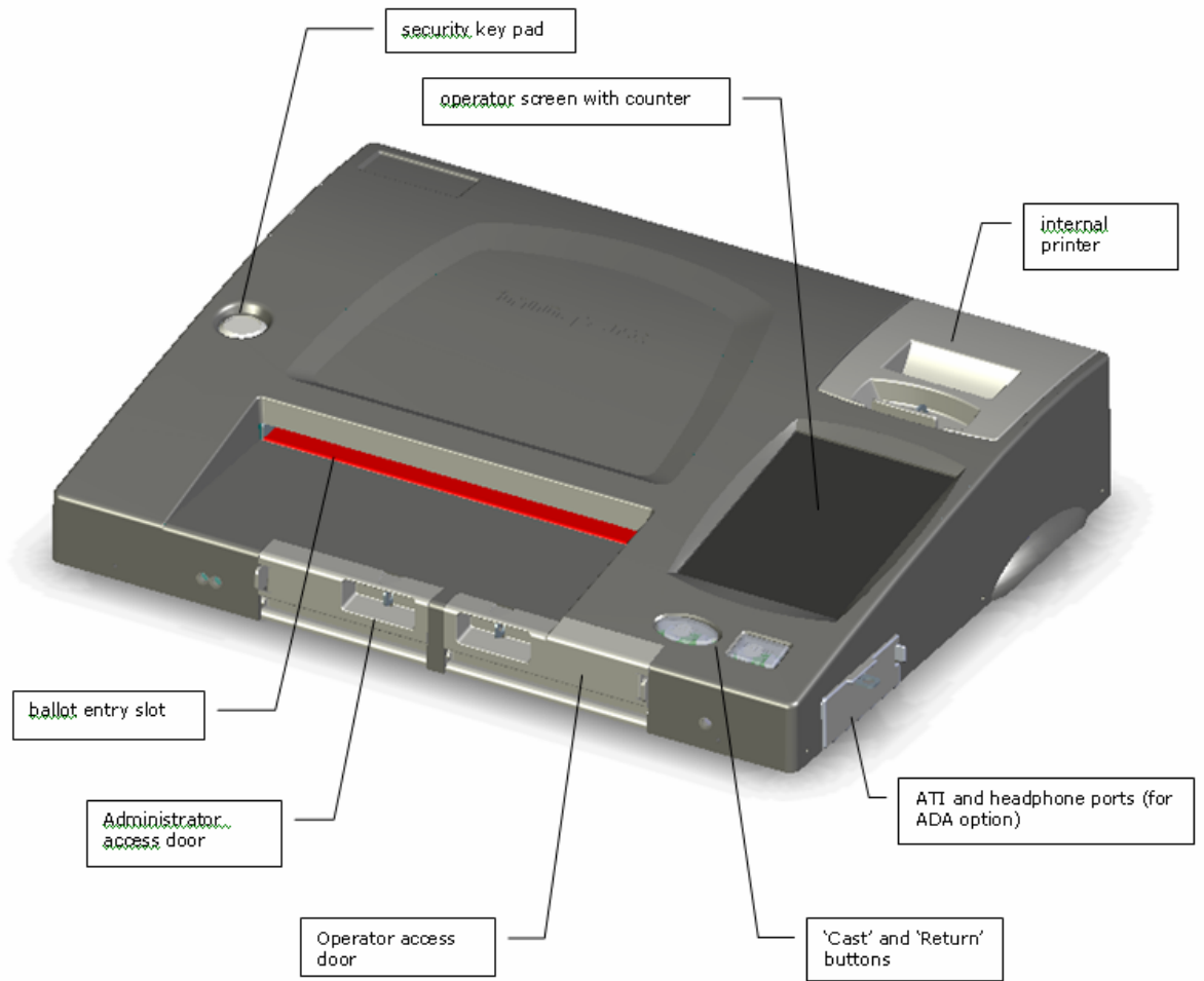
Figure 1: ImageCast Scanning Unit
